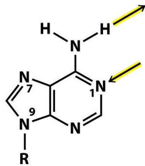
(Deoxy)Adenosine
