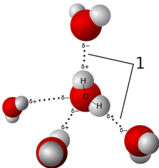
Figure 1c Hydrogen bonds among water molecules
