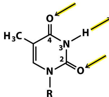
(Deoxy)Thymidine
