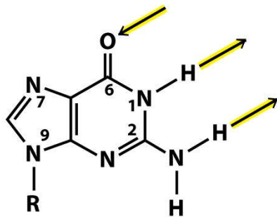
(Deoxy)Guanosine
