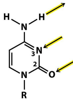
(Deoxy)Cytidine
